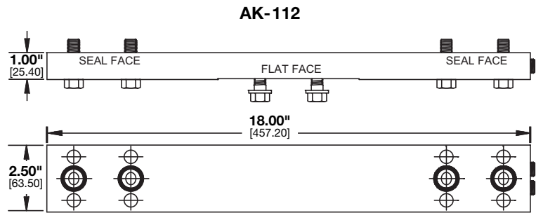
Co-Equal adapter mounts parallel to pipeline Dual ΔP, dual custody or bi-directional applications
