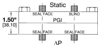
AK-023 ΔP to Static Adapter Stacks Static Transmitter on top of ΔP Transmitter
